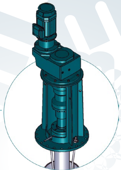
Sealing system and flange fixing
